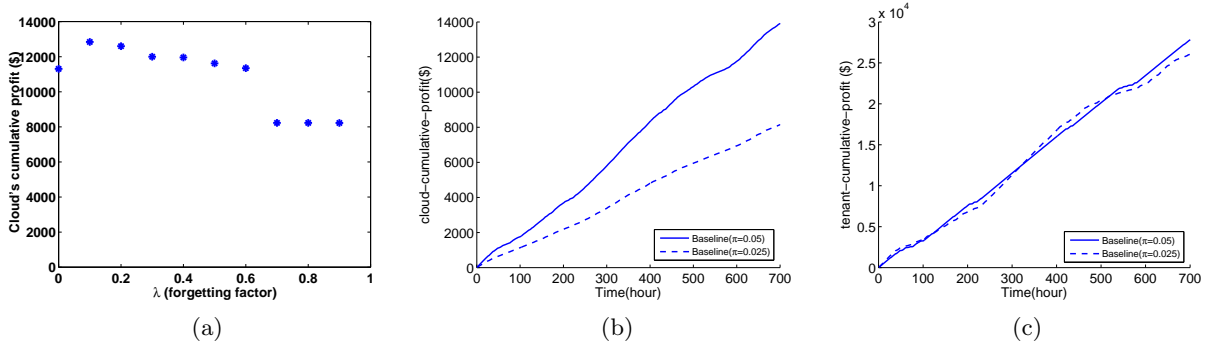
Figure 9: Scenario II: (a) Cloud's cumulative profit under PW-40- \lambda , \lambda \in [0, 0.9] . (b) Cloud's cumulative profit under Baseline with different delay costs \pi = 0.025, 0.05 . (c) Tenant's cumulative profit under Baseline with \pi = 0.025, 0.05 .
